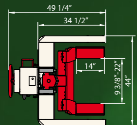
Adjustable fork
